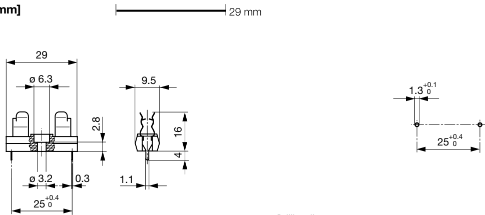
Drilling diagram
