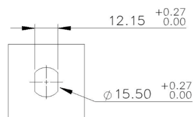
MOUNTING HOLE REQUIREMENTS
