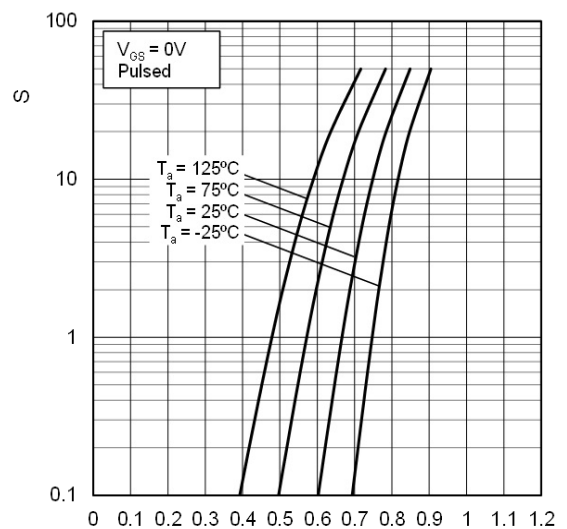
Fig.20 Source Current vs. Source Drain Voltage
