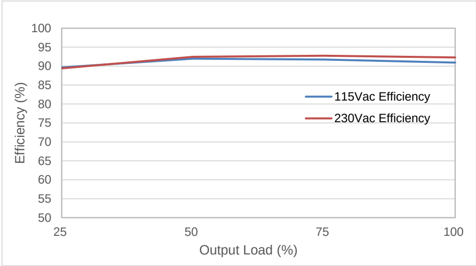
Fig 1. ADT-150A24AA Efficiency versus Output Load
