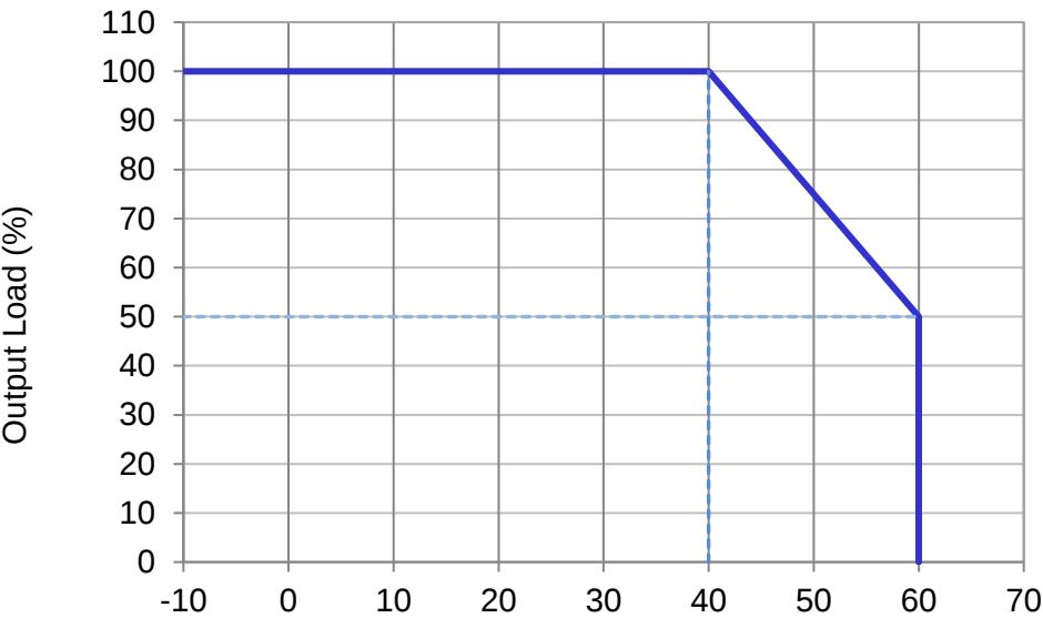
Fig. 2 De-rating for All Mounting Orientation > 40°C de-rate power by 2.5% / °C
