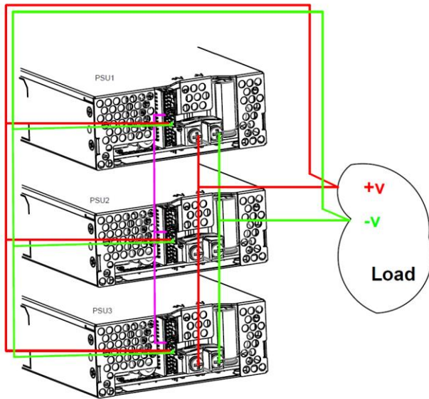
Parallel Connection without Remote Sense
