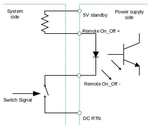
Fig. 12 Remote On_Off Connection
