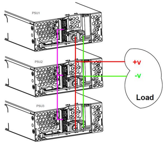
Parallel Connection with Remote Sense
