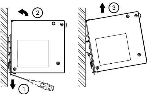
Fig. 3.2 Dismounting
