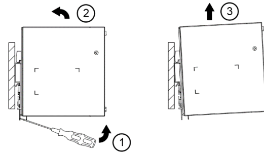
Fig. 3.2 Dismounting
