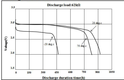
Discharge Characteristics
