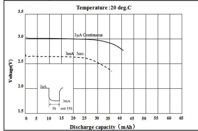
Pulse Discharge Characteristics
