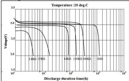
Discharge Characteristics
