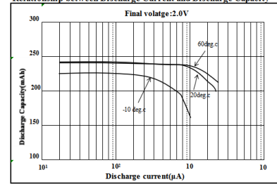
Relationship between Discharge Current and Discharge Capacity
