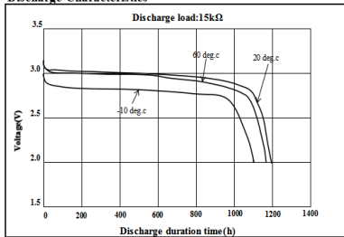
Discharge Characteristics
