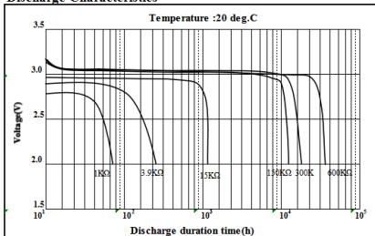
Discharge Characteristics
