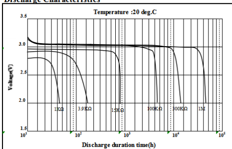
Discharge Characteristics
