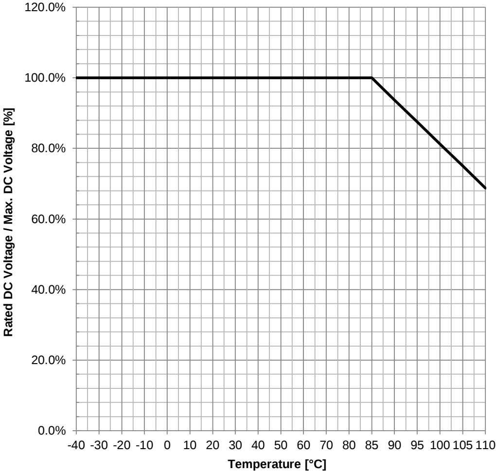
Rated DC Voltage vs. Temperature:
