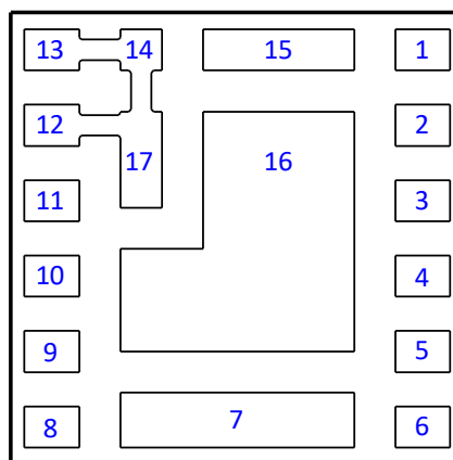
Figure 2 Pin layout (bottom view)
