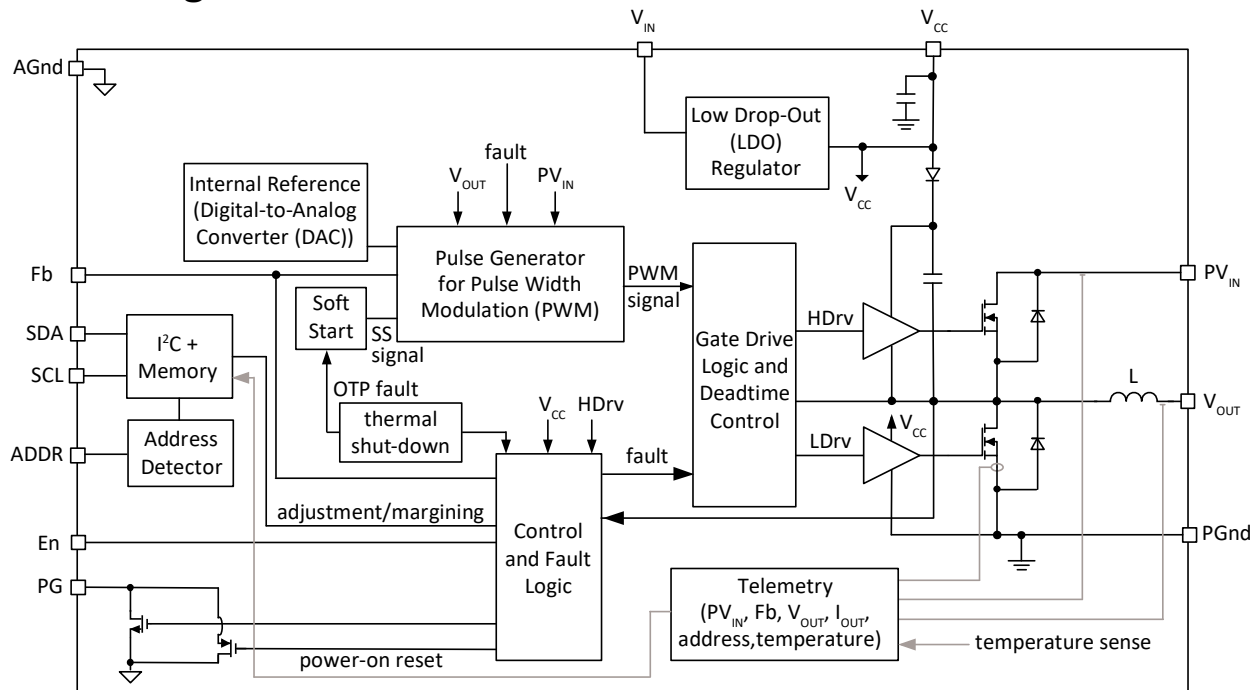
Figure 3 FS1603A \mu POL™
