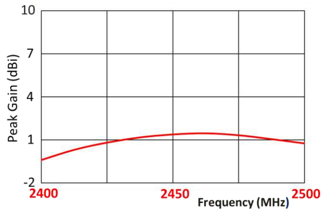
Peak Gain
