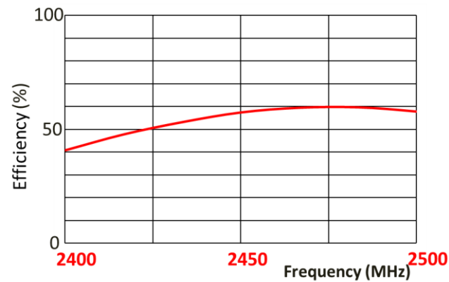
Efficiency
