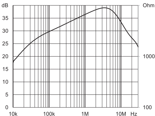
RT8x21-32-12M8
