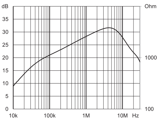
RT8x21-63-4M4
