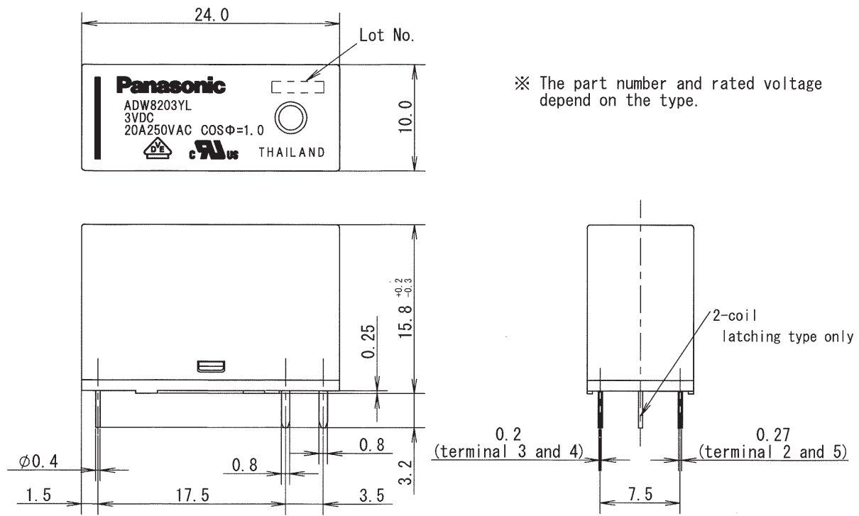
External dimensions (Tolerance: \pm 0.3 )
