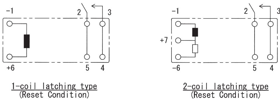
Schematic (Bottom view) (Reset condition)
