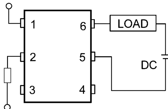
Fig. 14.2 B connection
