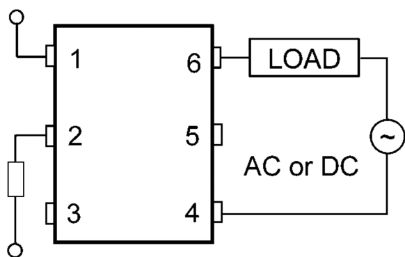
Fig. 14.1 A connection
