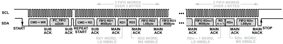
Figure 14. I2C FIFO Read (N 12-Bit Words); Sub Stands for Subordinate
