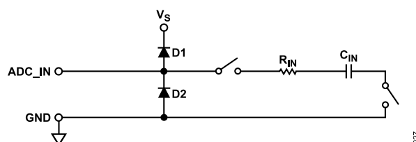
Figure 44. Equivalent Analog Input Circuit
