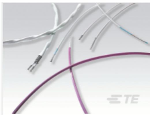
TE Part #CAT-55A-TC-H26 General Purpose Hookup Wire: Tin Coated Copper Wire, 26 AWG
