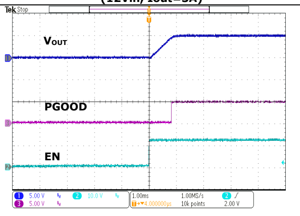
FIG.26 Turn-on (12Vin, Iout=3A)
