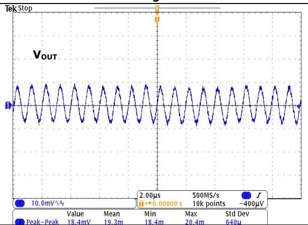
FIG.24 Output Ripple (12Vin, Iout=3A)
