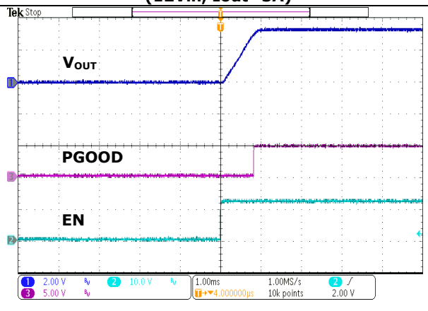
FIG.20 Turn-on (12Vin, Iout=3A)
