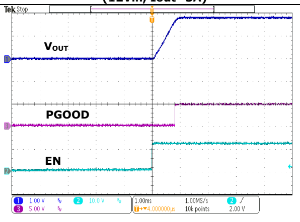
FIG.14 Turn-on (12Vin, Iout=3A)
