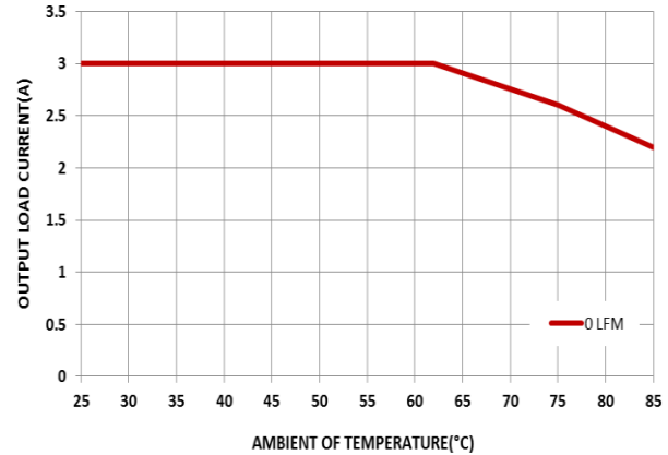
FIG.22 De-rating Curve at 12Vin
