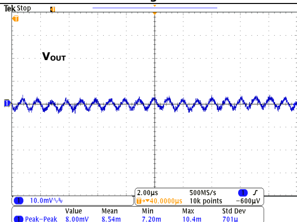
FIG.12 Output Ripple (12Vin, Iout=3A)
