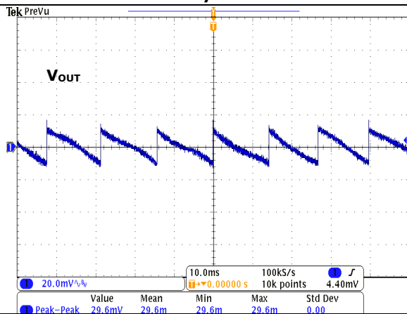
FIG.23 Output Ripple (12Vin, Iout=0A)
