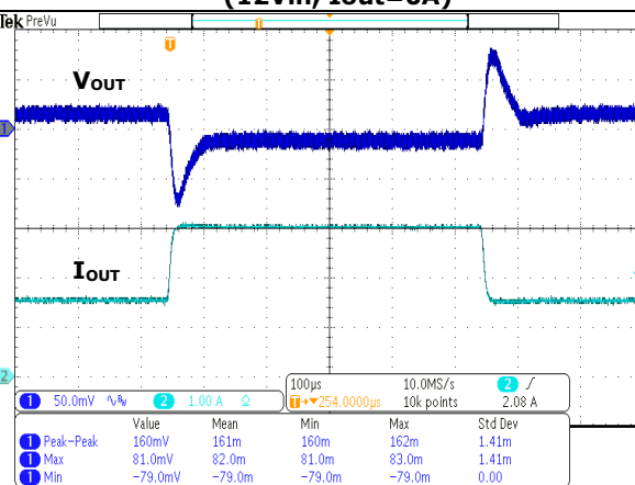
FIG.25 Transient Response (12Vin, 50% to 100% Load Step)
