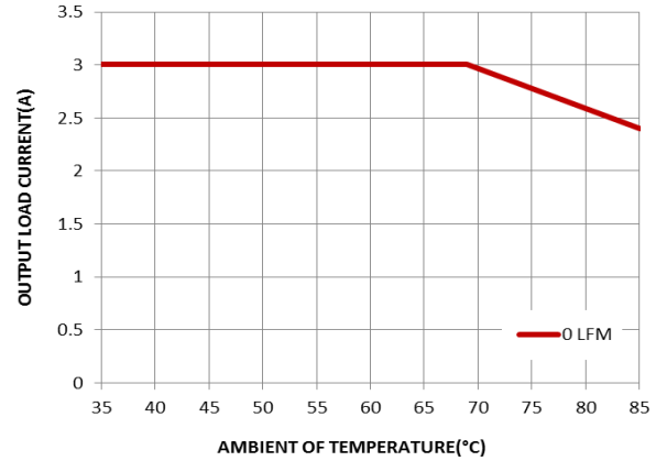
FIG.10 De-rating Curve at 12Vin
