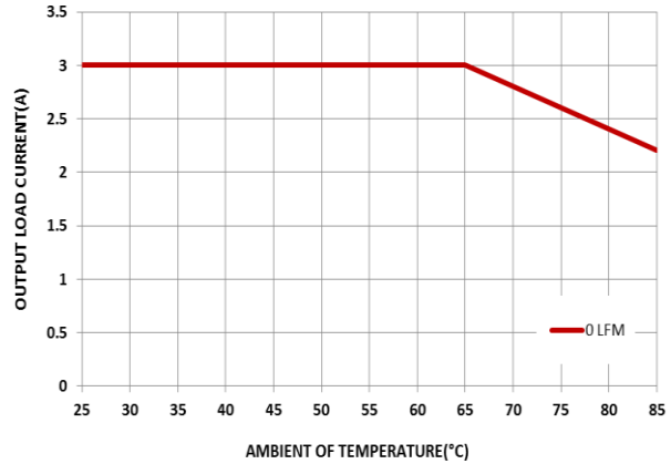
FIG.16 De-rating Curve at 12Vin
