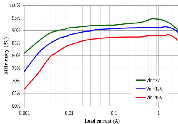
FIG.21 Efficiency V.S. Load Current
