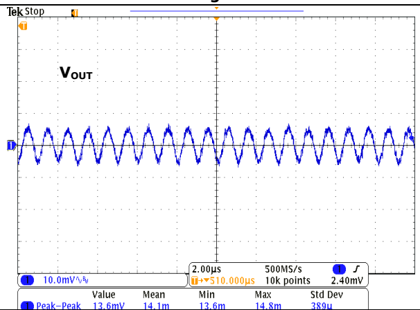
FIG.18 Output Ripple (12Vin, Iout=3A)
