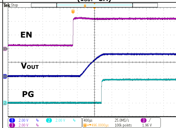
FIGURE 8 Turn-On (V IN =5.0V, I OUT =3A)
