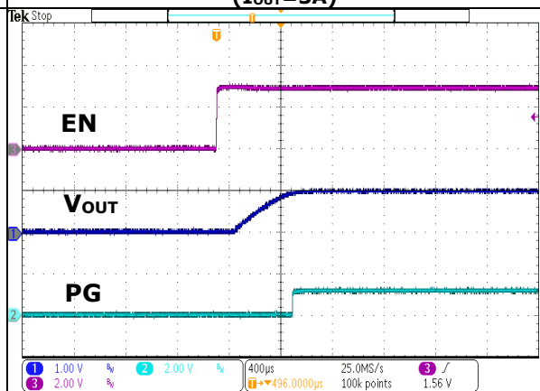
FIGURE 20 Turn-On ( V_{IN}=3.3\text{V}, I_{OUT}=3\text{A} )
