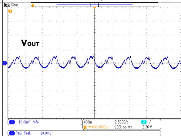
FIGURE 6 Output Ripple at 5.0V IN (I OUT =3A)
