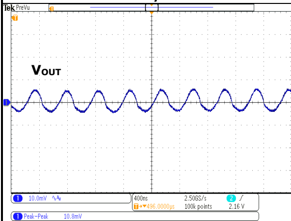
FIGURE 5 Output Ripple at 5.0V IN (I OUT =0A)
