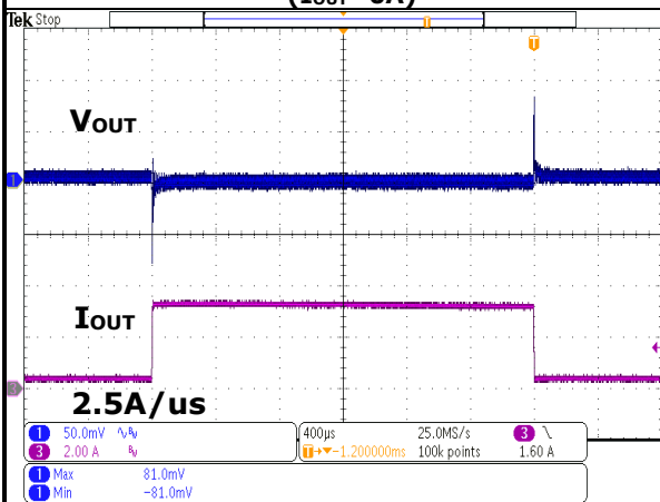
FIGURE 7 Transient Response (V IN =5.0V, I OUT =0.3A~3A)
