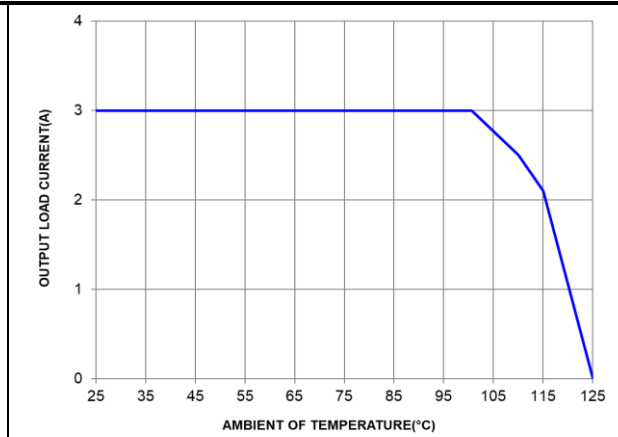
FIGURE 16 De-rating Curve at 3.3V IN
