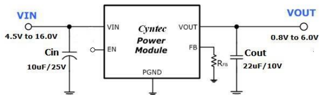
FIG.1 TYPICAL APPLICATION CIRCUIT
