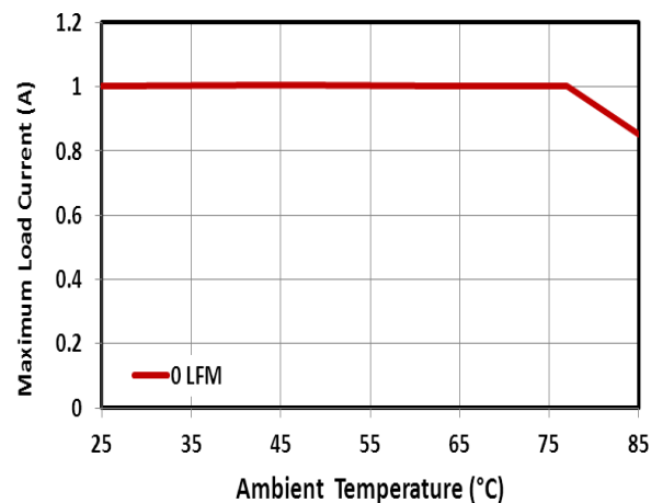
FIG.4 DE-RATING CURVE AT 3.3VIN
