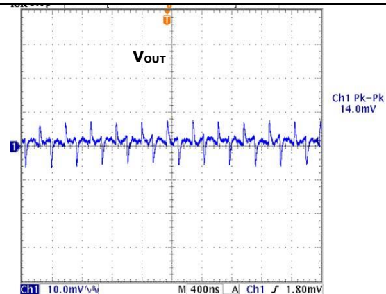
FIG.6 OUTPUT RIPPLE (3.3VIN, I_{OUT}=1000\text{mA} )
