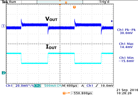
FIG.13 TRANSIENT RESPONSE (5.0VIN, 50% to 100% LOAD STEP)
