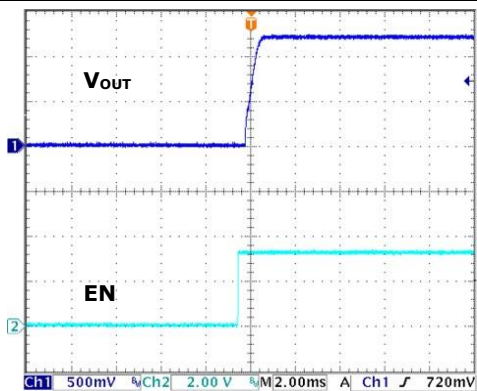
FIG.14 TURN-ON (3.3VIN, IOUT=1000mA)
