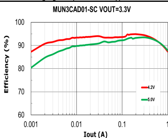
FIG.33 EFFICIENCY V.S. LOAD CURRENT
