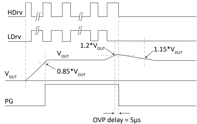
Figure 11 Illustration of latched OVP
