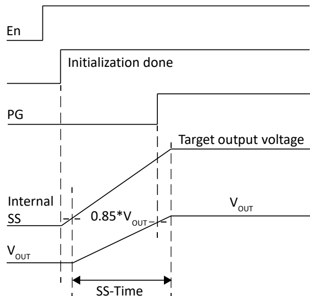
Figure 7 Theoretical operational waveforms during soft-start
