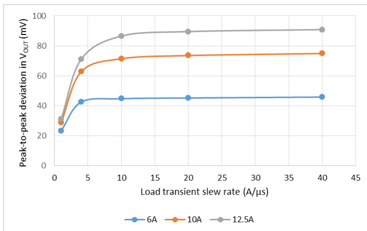
Figure 16 Peak-to-peak voltage deviation ( V_{OUT} = 1.2V )
