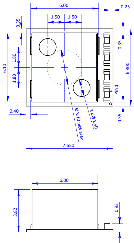
Figure 33 Dimensioned drawings
