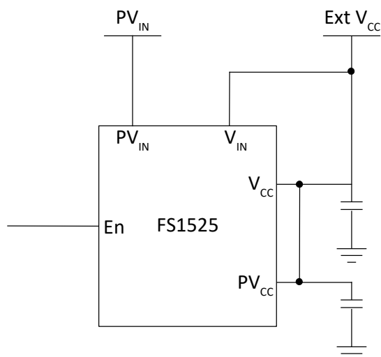
Figure 6 Using an external bias voltage
