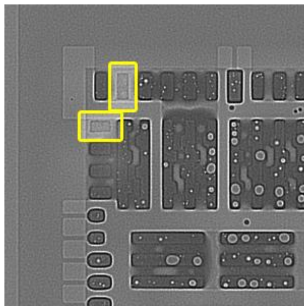
Figure 37 X-ray showing incorrectly soldered pads
