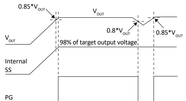
Figure 13 PG signal when PGControl bit=0
