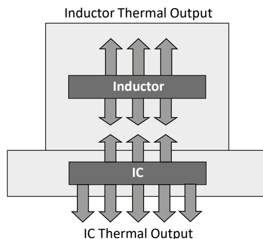
Figure 31 Heat sources in the FS1525
