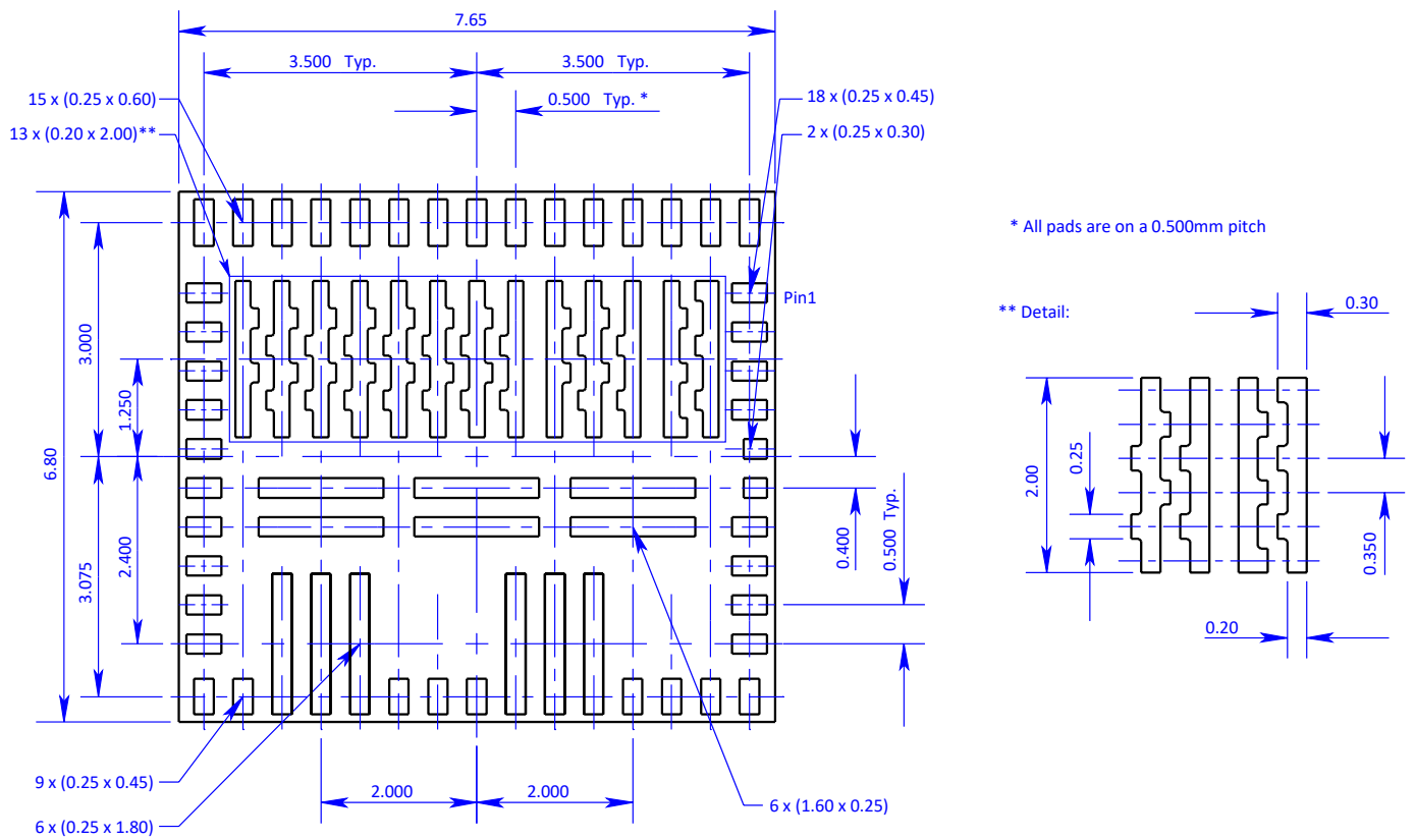
Figure 34 Package footprint
