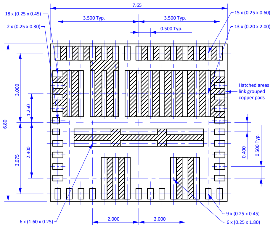
Figure 38 Copper pads and tracks
