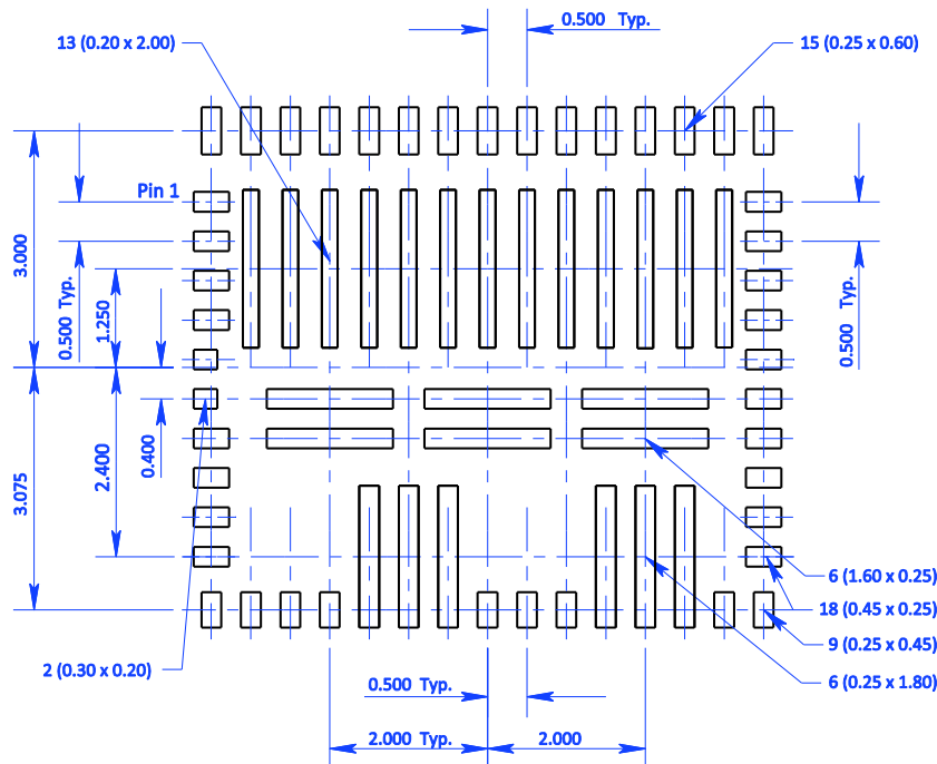
Figure 40 Solder stencil
