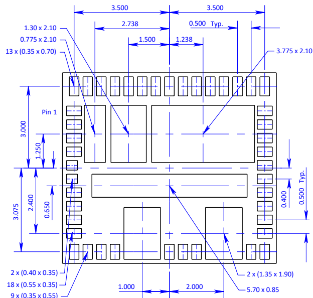
Figure 35 Solder mask
