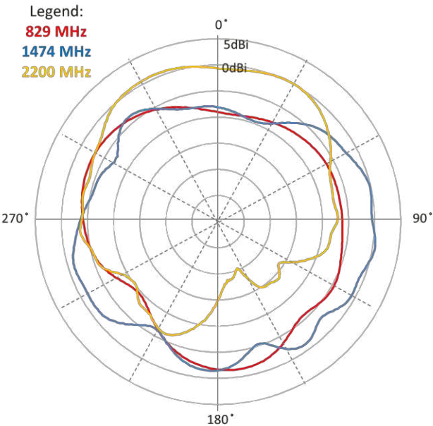
Elevation 1(XZ)
