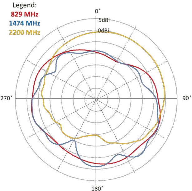
Elevation 2(YZ)
