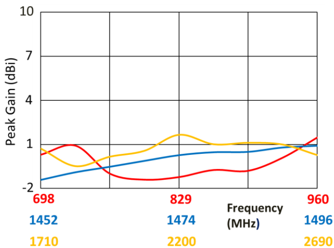
Peak Gain
