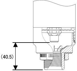
<Direct Mount Bracket part section>
