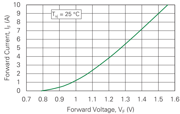
Figure 1. Typical On-state Current vs. On-state Voltage
