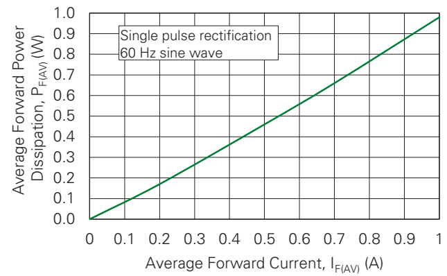
Figure 2. Typical Power Dissipation vs. Average Forward On-state Current
