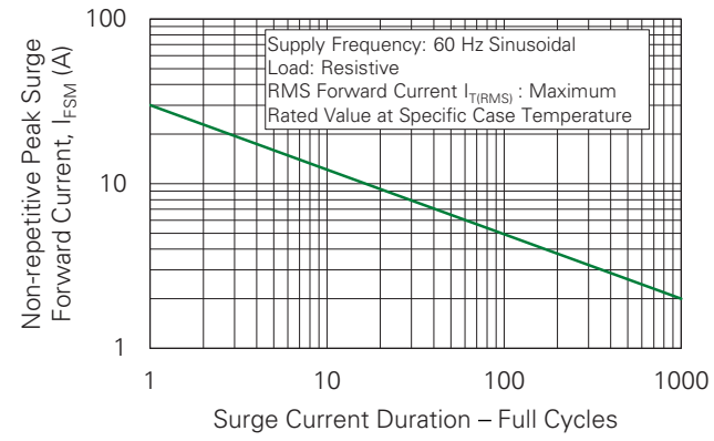
Figure 4. Surge Peak On-state Current vs. Number of Cycles
