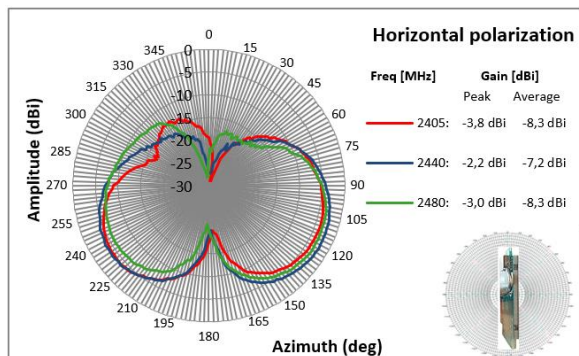
Figure 20. Radiation pattern for XZ-plane, horizontal polarization
