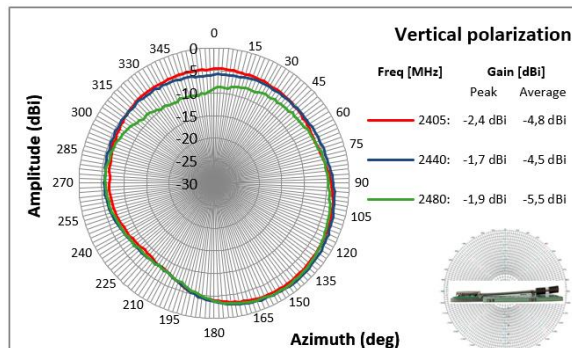
Figure 19. Radiation pattern for XY-plane, vertical polarization
