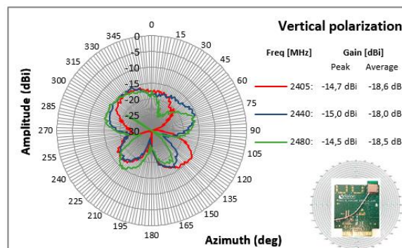
Figure 23. Radiation pattern for YZ-plane, vertical polarization
