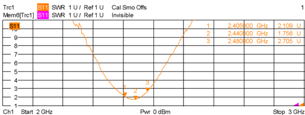
Figure 15. VSWR with module installed in center (position #2) of the evaluation board
