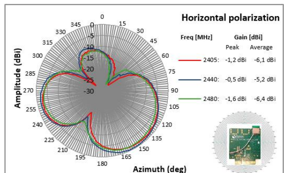
Figure 22. Radiation pattern for YZ-plane, horizontal polarization
