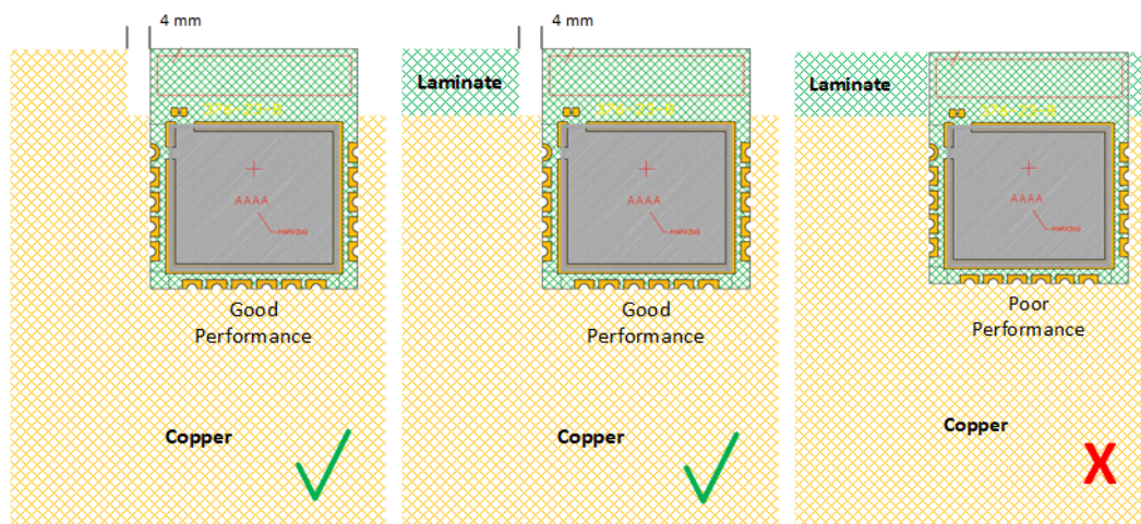
Figure 12. Antenna performance in proximity of copper (left), laminate (middle), and laminate under antenna (right) The actual TINY™ module evaluation board layout that has been used to conduct measurements is shown in Figure 13.
