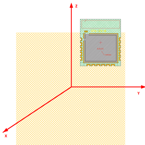
Figure 17. Measurement plane definition
