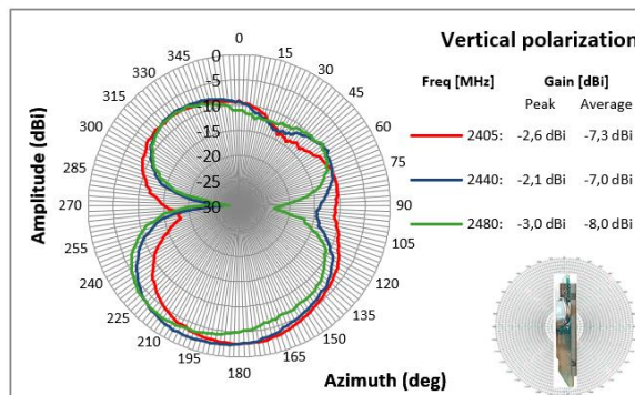
Figure 21. Radiation pattern for XZ-plane, vertical polarization
