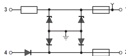
Figure 3.2.1.1 – ISBS-STD-06 schematic
