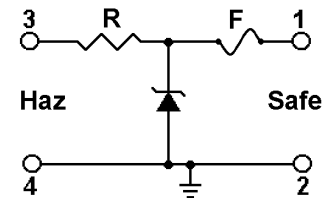
Figure 2.2.1 - Basic zener barrier schematic
