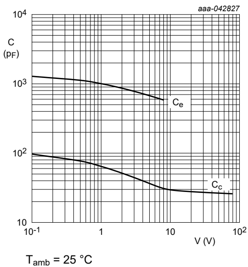
Fig. 11. Input/output capacitance as a function of input/output voltage
