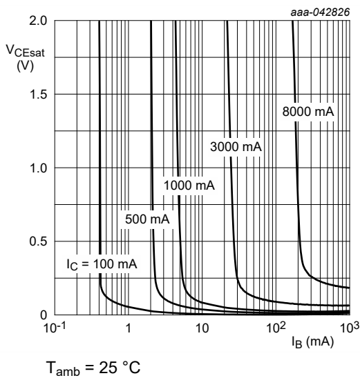
Fig. 10. Collector-emitter saturation region as a function of base current; typical values
