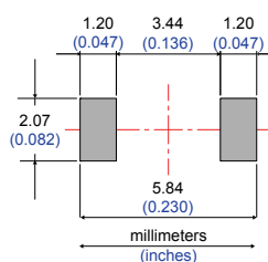
Figure 11. Footprint recommendations, dimensions in mm (inches)
