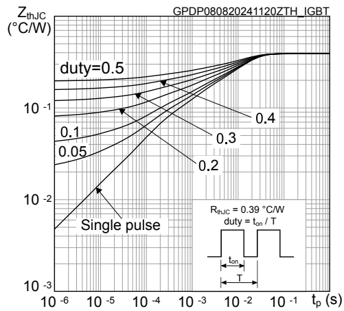
Figure 19. IGBT maximum transient thermal impedance
