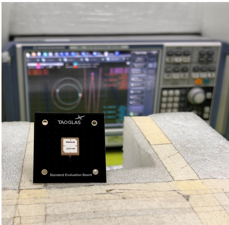
VNA Test Set-up
