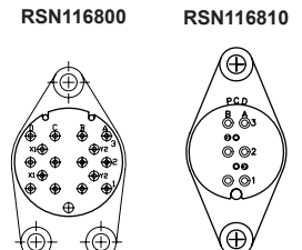
Socket Configurations
