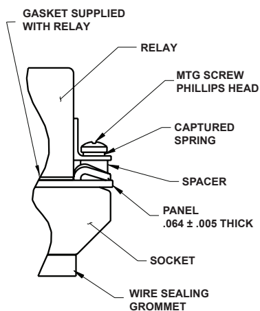
Mounting Hardware
