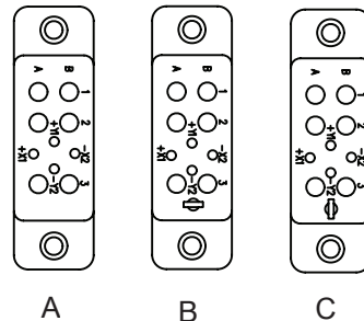
Socket Configurations
