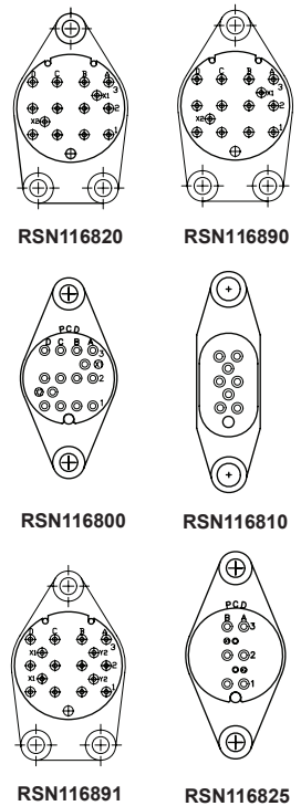
Socket Configurations
