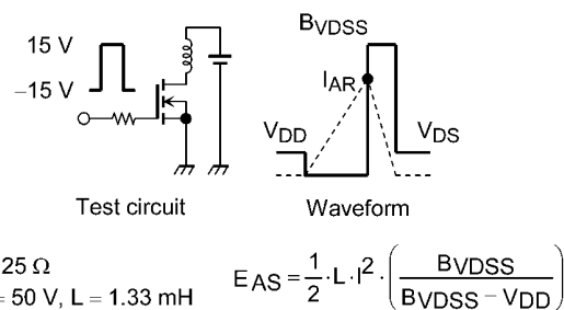
Fig. 8.16 Test Circuit/Waveform
