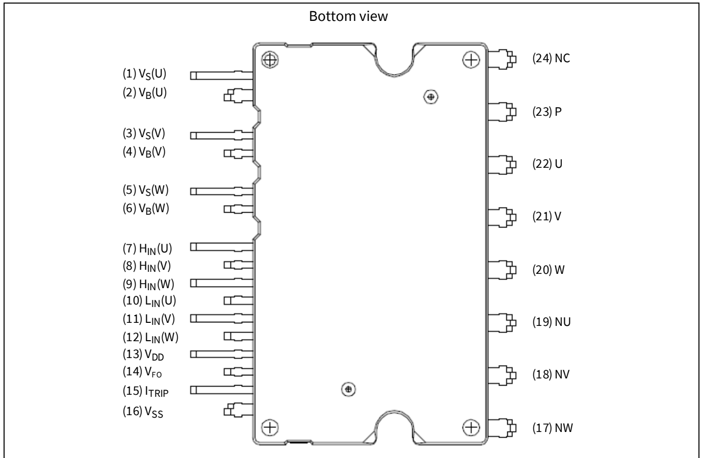
Figure 2 Pin assignment
