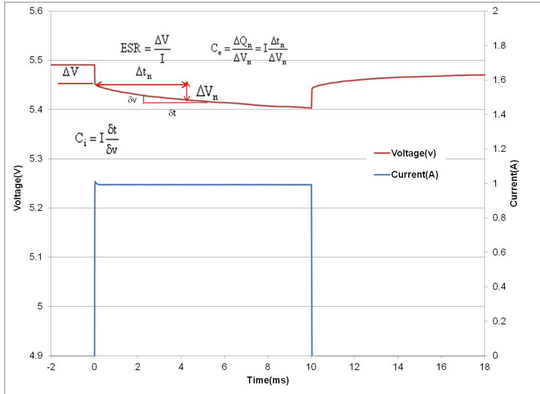
Fig 1: Effective capacitance, instantaneous capacitance and ESR for an HS208
