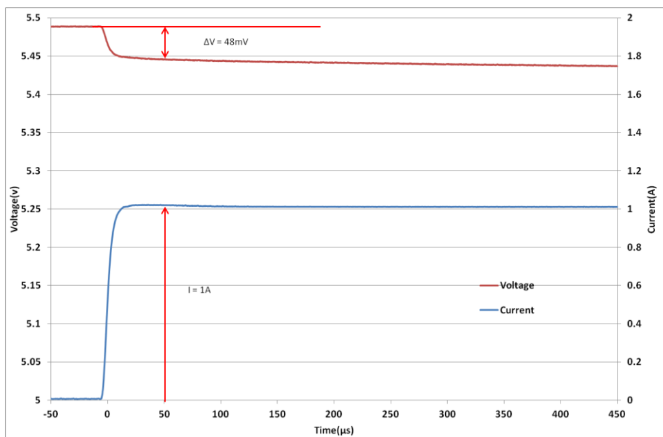
Fig 3: Measurement of ESR for an HS208
