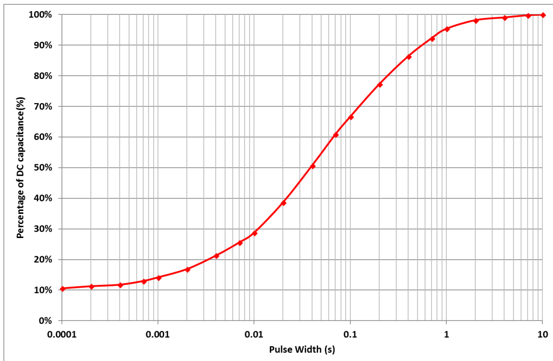
Figure 4: Effective Capacitance
