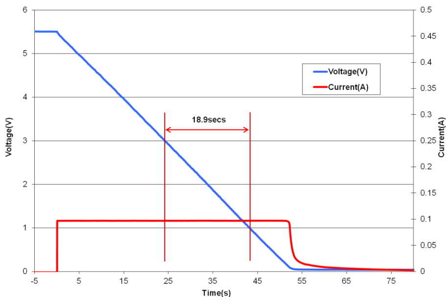
Fig 2: Measurement of DC Capacitance for an HS208
