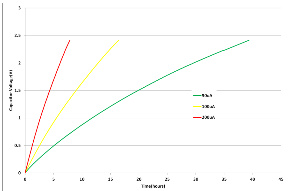
Fig 11: Charging an HS108 with low current
