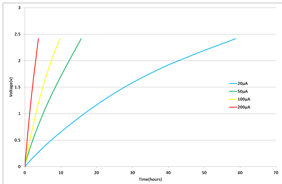
Fig 11: Charging an HW103 with low current
