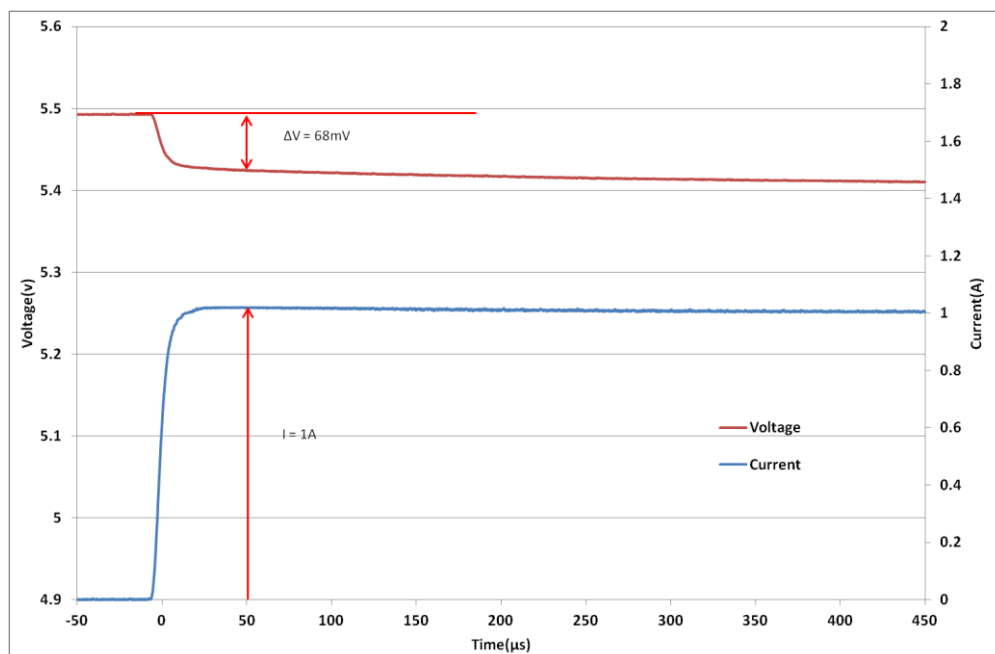
Fig 3: Measurement of ESR for an HW203
