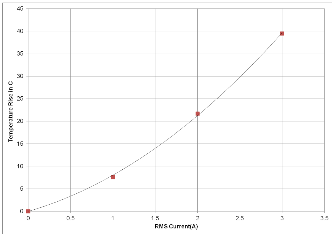
Fig 12: Temperature rise in HW201 with RMS current
