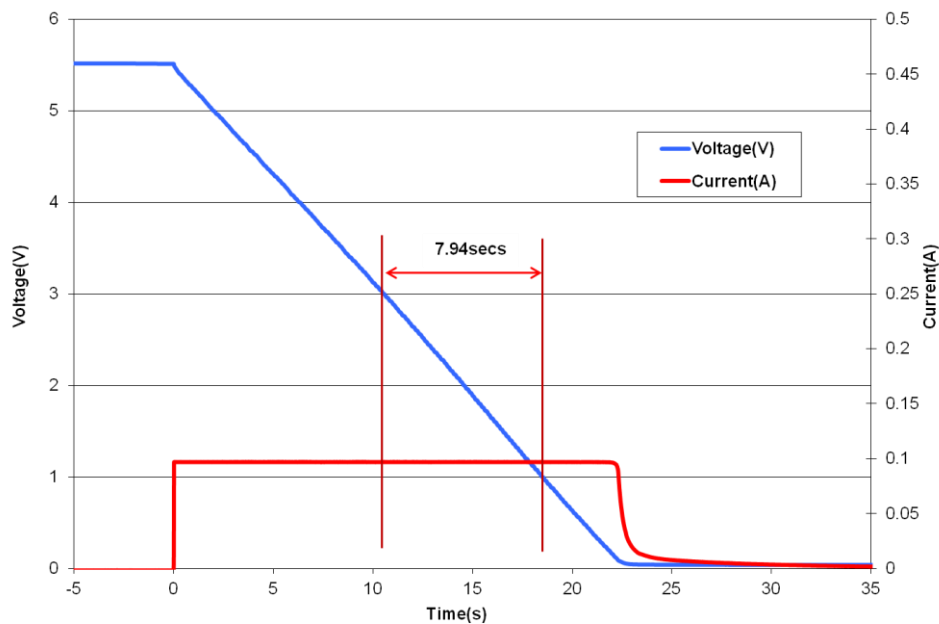
Fig 2: Measurement of DC Capacitance for an HW201
