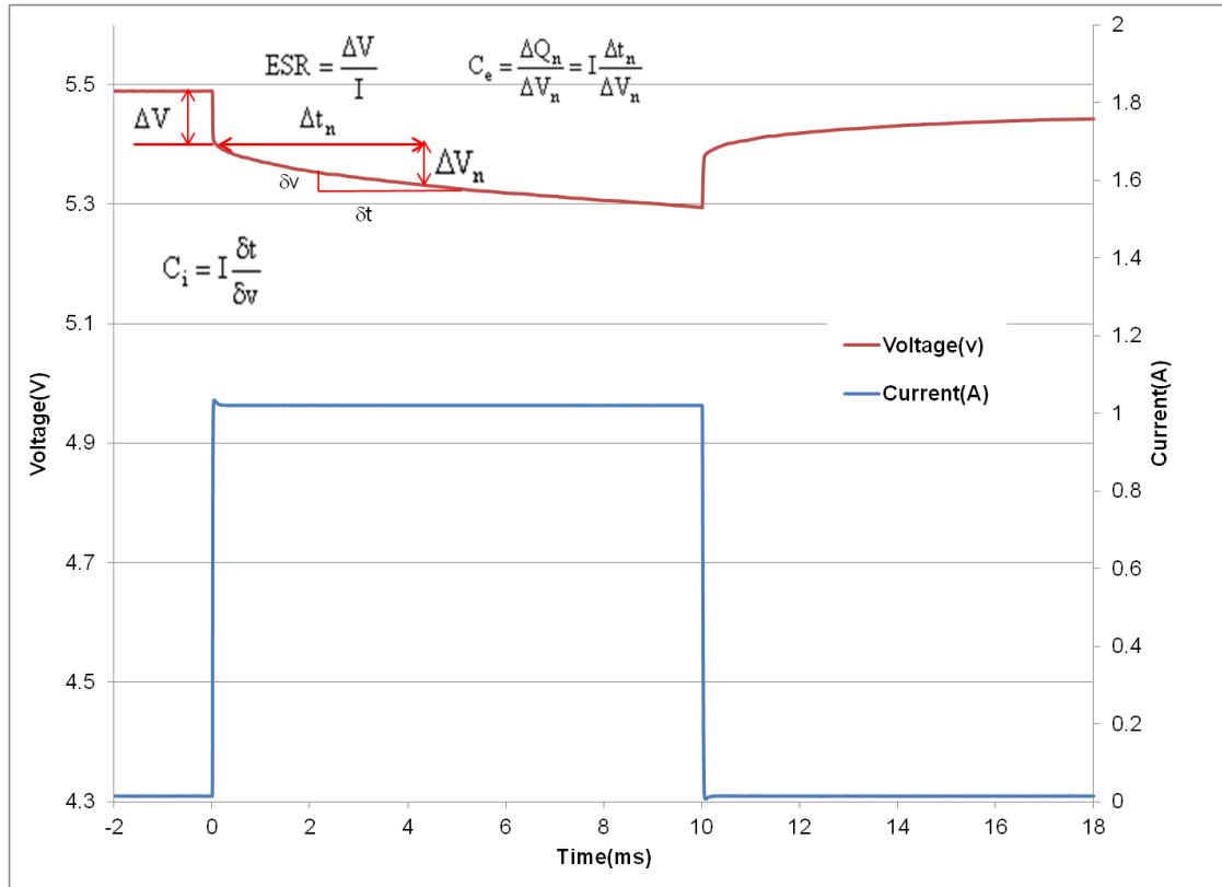
Fig 1: Effective capacitance, instantaneous capacitance and ESR for an HW201
