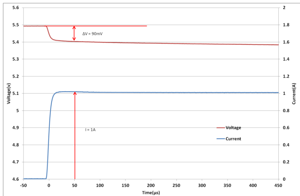
Fig 3: Measurement of ESR for an HW201
