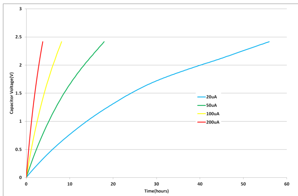
Fig 11: Charging an HW101 with low current
