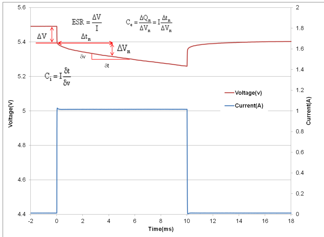
Fig 1: Effective capacitance, instantaneous capacitance and ESR for an HW209
