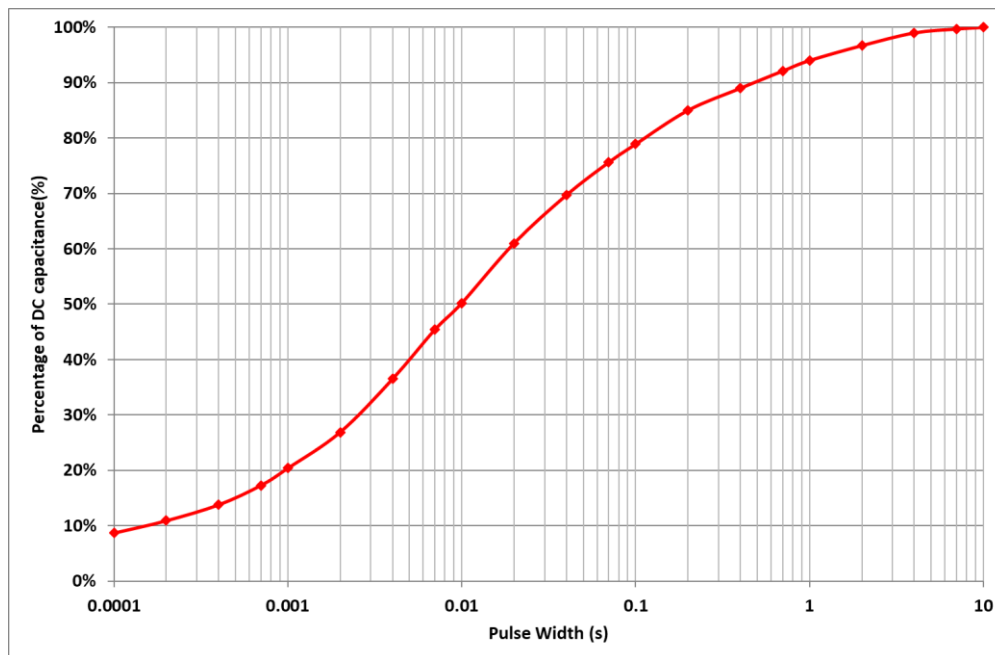
Fig 4: Effective Capacitance
