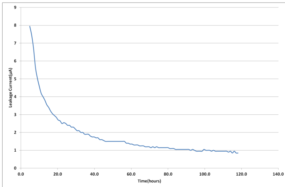
Fig 10: Leakage Current
