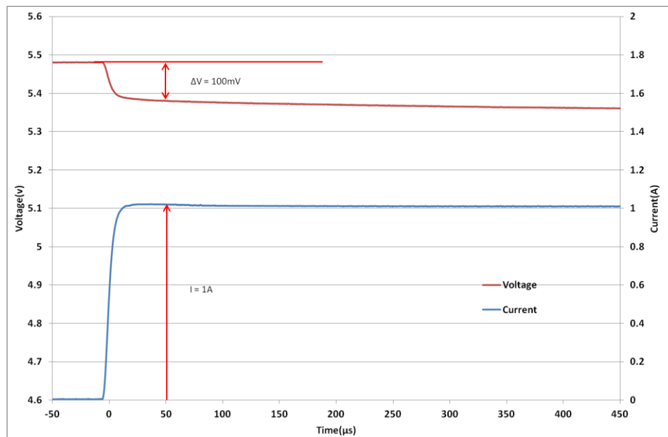
Fig 3: Measurement of ESR for an HW209
