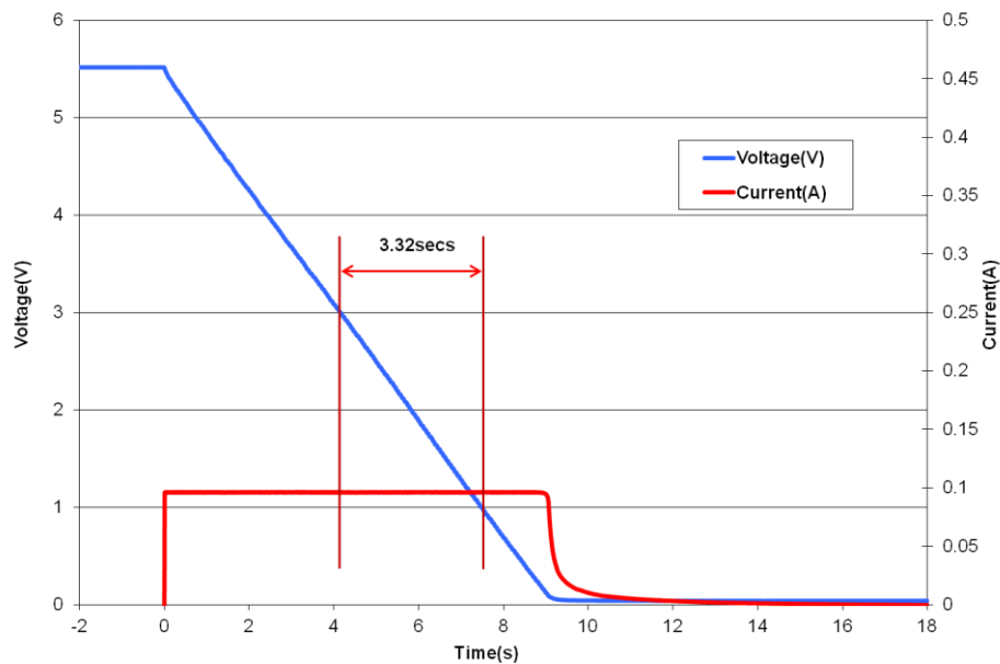
Fig 2: Measurement of DC Capacitance for an HW209
