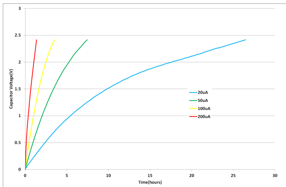
Fig 11: Charging an HW109 with low current
