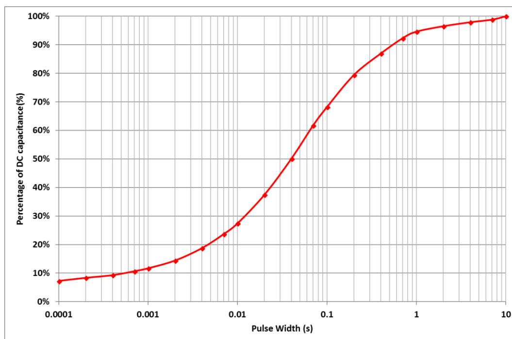
Figure 4: Effective Capacitance
