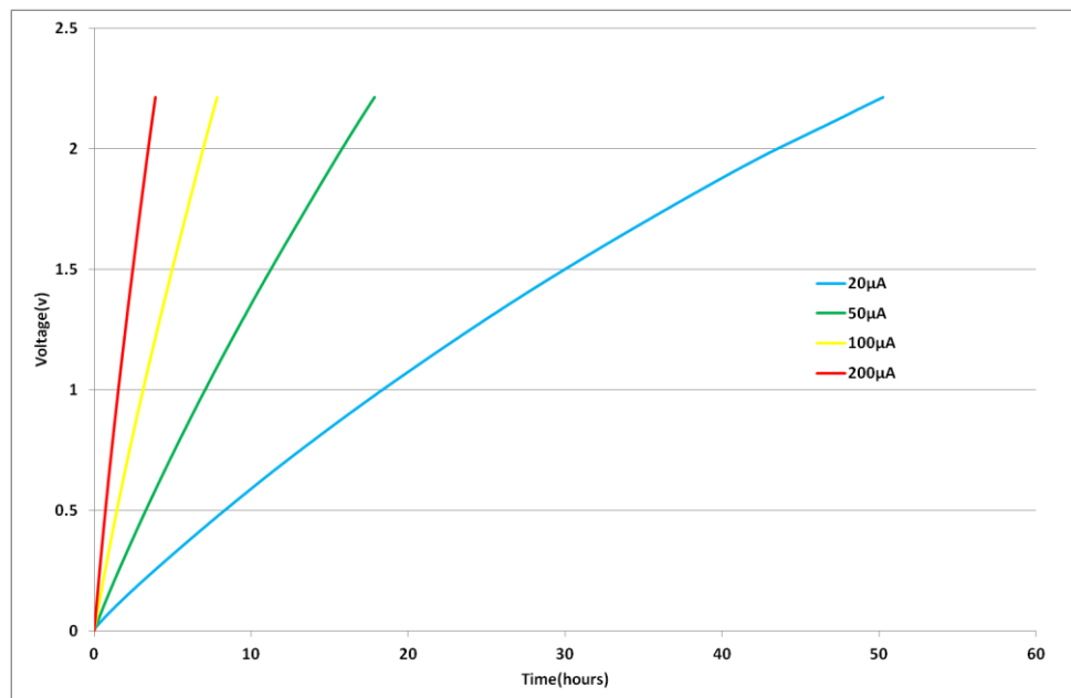
Fig 11: Charging a GW103 with low current
