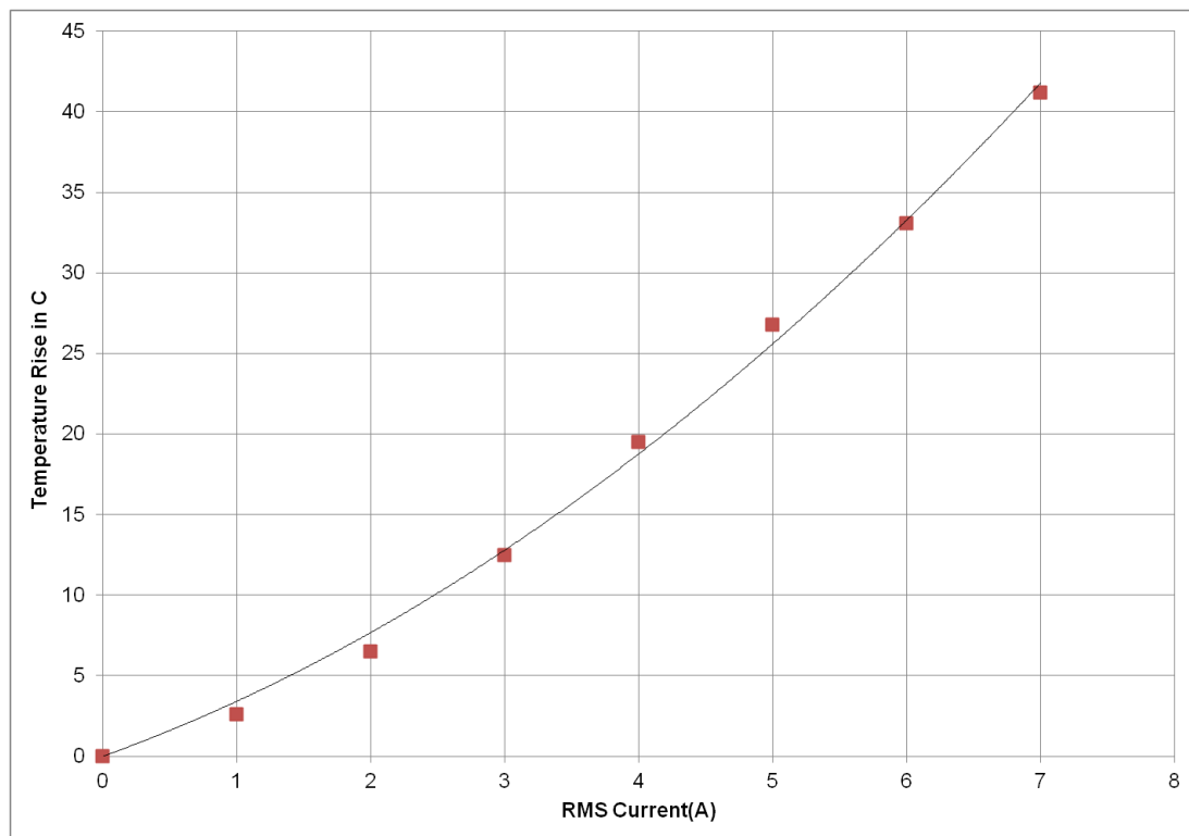
Fig 12: Temperature rise in GW203 with RMS current
