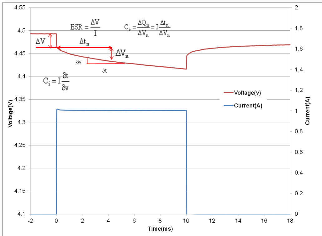
Fig 1: Effective capacitance, instantaneous capacitance and ESR for a GW203
