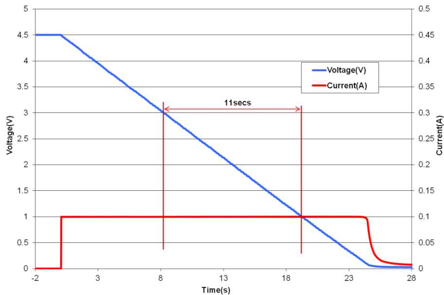
Fig 2: Measurement of DC Capacitance for a GW203
