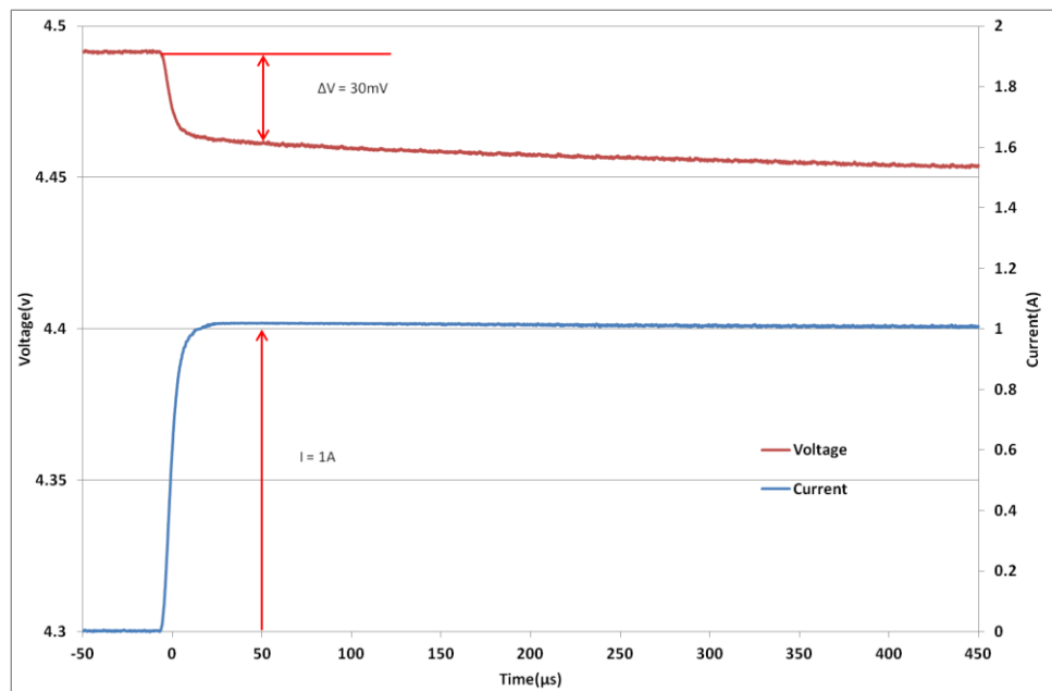
Fig 3: Measurement of ESR for a GW203
