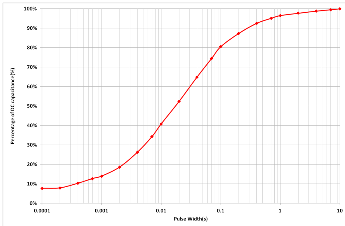
Figure 4: Effective Capacitance
