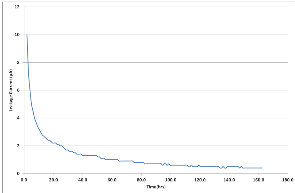
Fig 10: Leakage Current
