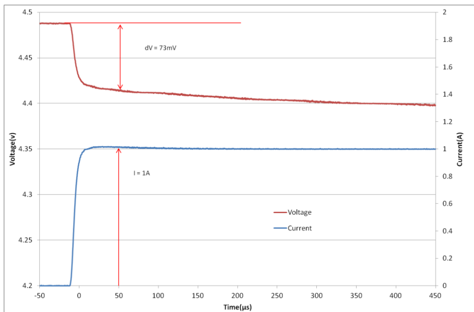
Fig 3: Measurement of ESR for a GA209
