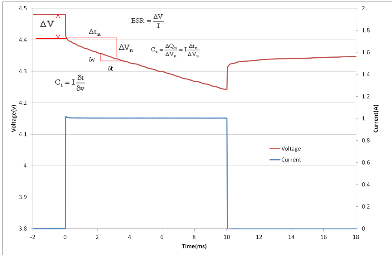
Fig 1: Effective capacitance, instantaneous capacitance and ESR for a GA209
