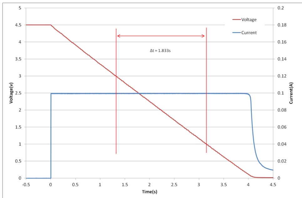
Fig 2: Measurement of DC Capacitance for a GA209
