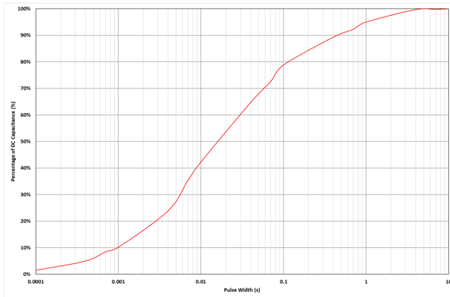
Fig 4: Effective Capacitance
