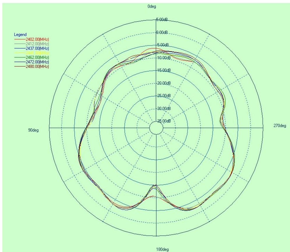
Figure 13-4. Antenna Radiation Pattern When \Phi = 90 Degrees
