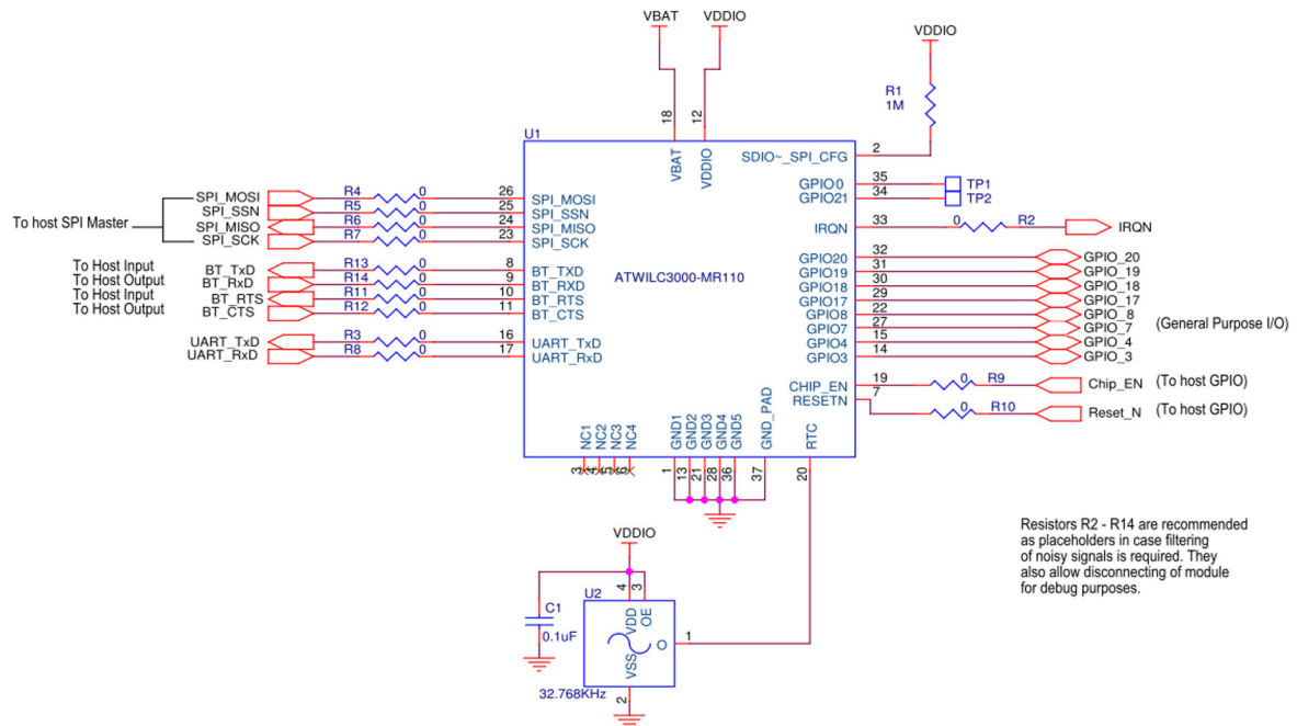
Figure 11-1. ATWILC3000-MR110xA Reference Schematic for SPI Operation
