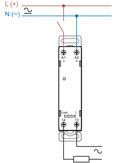
Single-phase connection (77.11/77.21)
