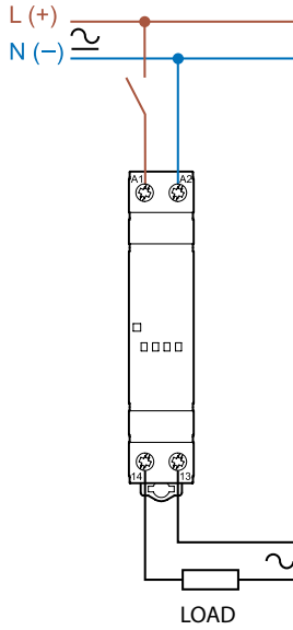
Single-phase connection (77.31...805x)
