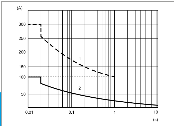
L77-8 Inrush peak current (AC) v inrush time 77.01.x.xxx.80xx
