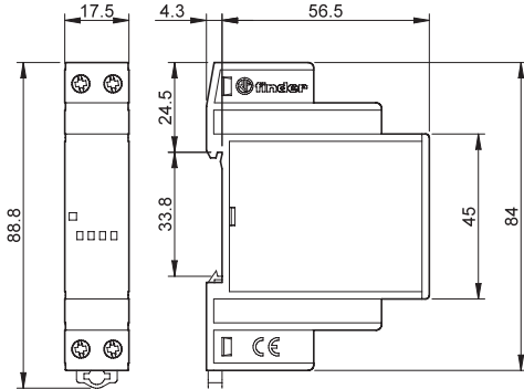
Type 78.25 Box clamp
