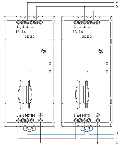
Series connection
