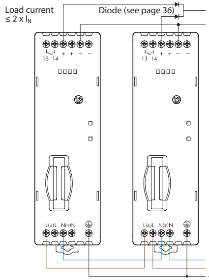
Parallel connection
