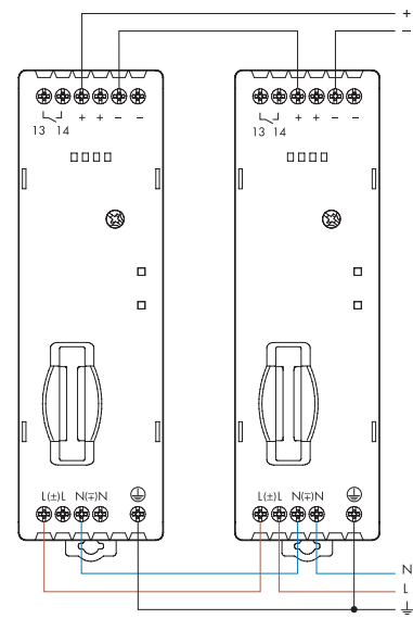
Series connection
