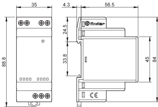
Type 78.36/78.50/78.60 Box clamp
