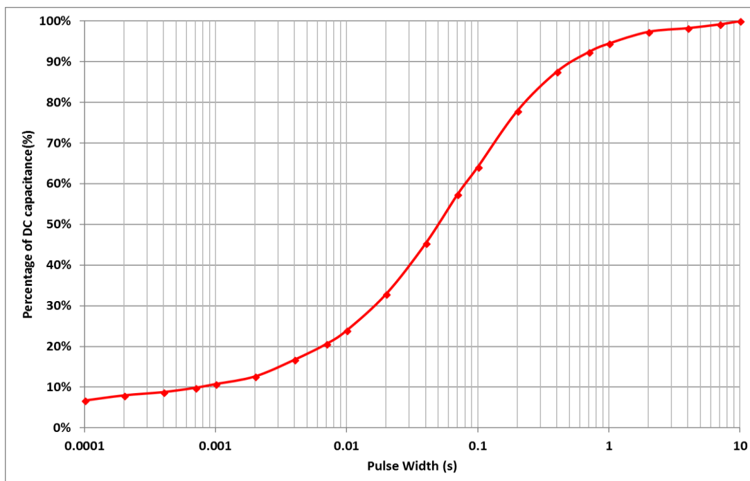
Figure 4: Effective Capacitance
