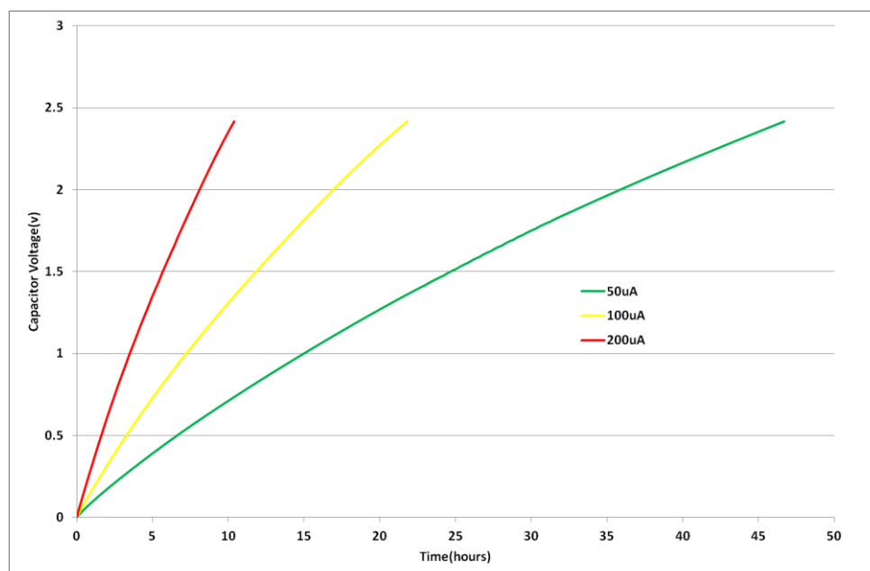
Fig 11: Charging an HS130 with low current
