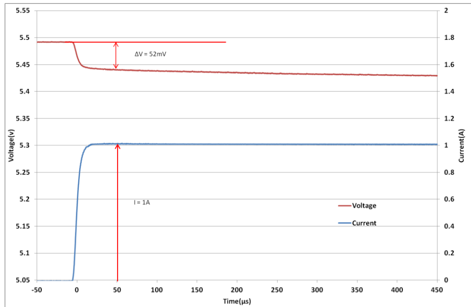
Fig 3: Measurement of ESR for an HS206
