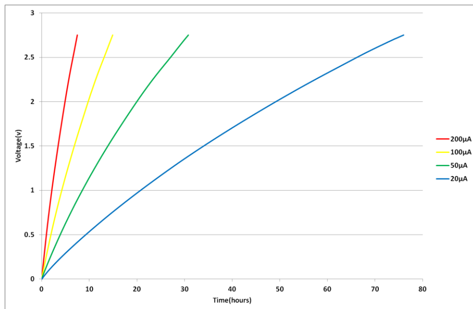
Fig 11: Charging an HS106 with low current
