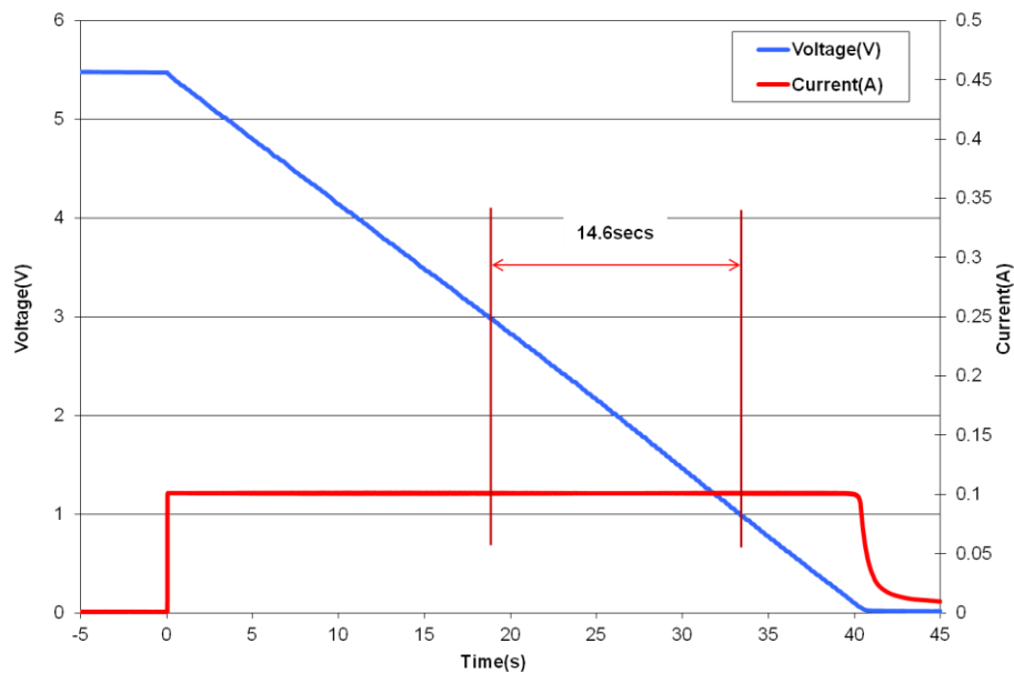
Fig 2: Measurement of DC Capacitance for an HS206
