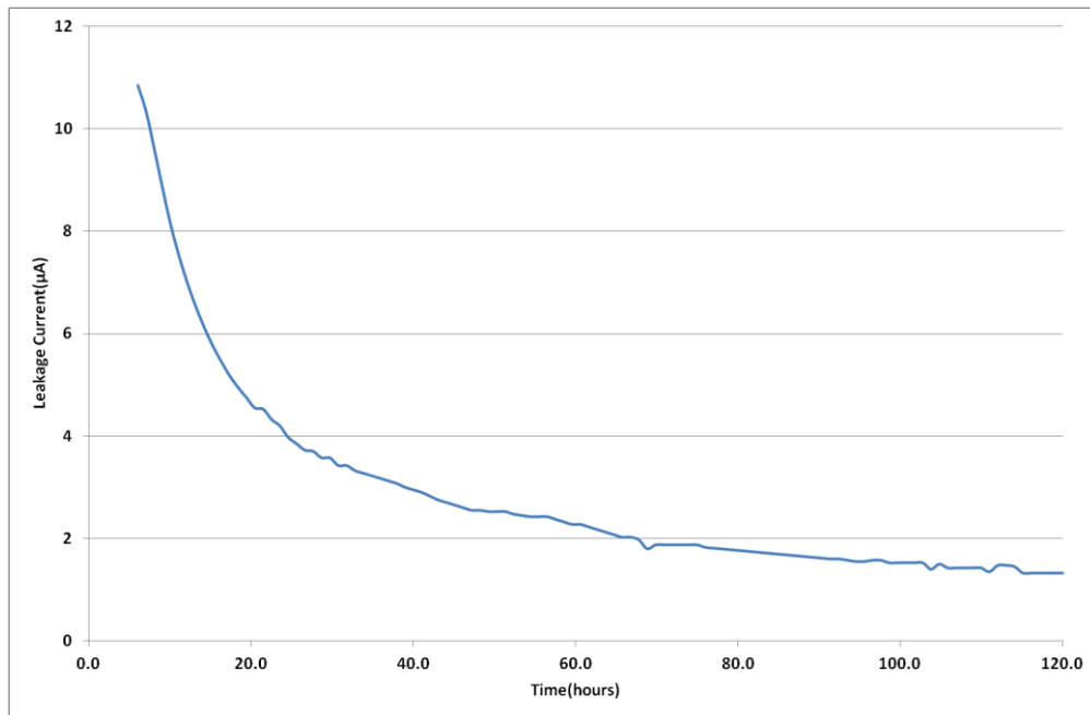
Fig 10: Leakage Current
