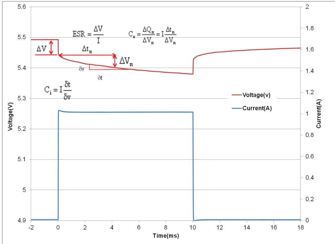
Fig 1: Effective capacitance, instantaneous capacitance and ESR for an HS206
